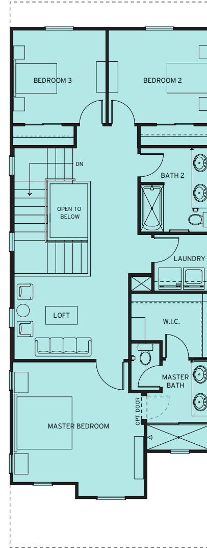
UPPER FLOOR
