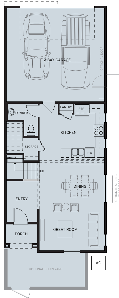
MAIN FLOOR
